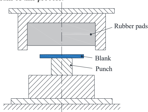
Fig. 2. Guerin process [8]
