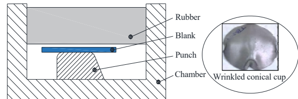
Fig. 15. Schematic representation of experimental set-up [17]
