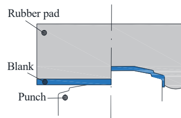
Fig. 16. Rubber Pad Forming (RPF) process schematization: flexible rubber die (rubber pad) and rigid tool (punch) [18]
