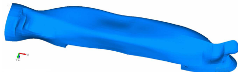
Fig.6.4 LPG carrier(B),H4(71),8.585Hz.
