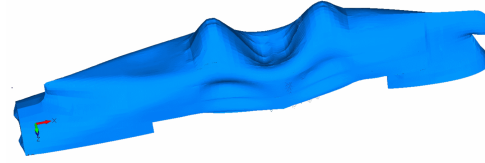
Fig.4.4 LPG carrier(B),V4(43),6.817Hz.
