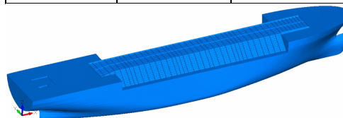
Fig.1 LPG ship, structural model [3].
