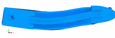
Fig.5.2 LPG carrier(F),H2(18),3.472Hz.
