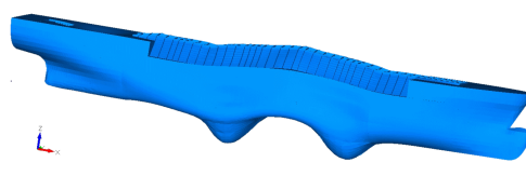
Fig.3.4 LPG carrier(F),V4(34),5.534Hz.
