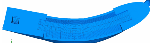
Fig.5.1 LPG carrier(F),H1(7),2.183Hz.
