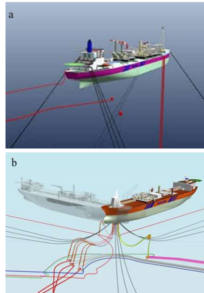
Figure 1 Spread moored floater (a) and turret moored floater (b) [16]
