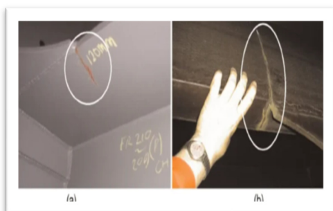
Fig.4 Cracks in ship structure caused by vibrations [6].
