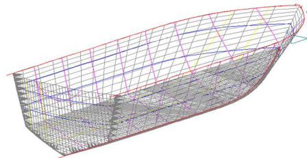
Fig. 3.8.d. Mono Hull 3D view
